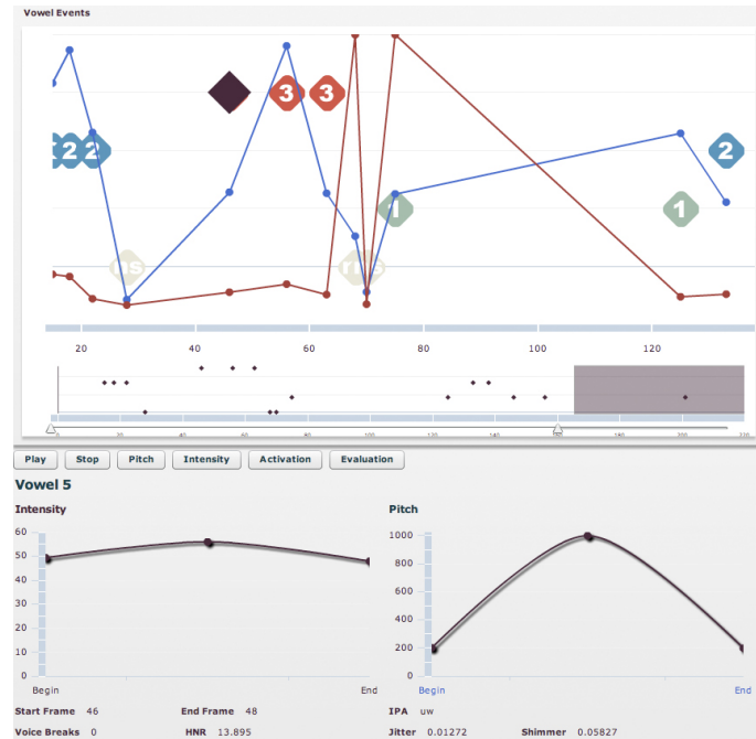
Fig. 2. Screen shot of the CorpVis asset viewer tool. This tool provides a visualization of all acoustic, linguistic and emotional data relating to a single asset. The user can also add annotations (not shown) that will update the corpora database.
